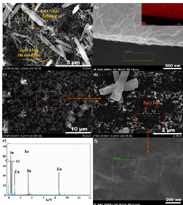
Figure 2. a) SEM micrograph of smaller ZnO Nanorods grown on PET and larger Nanorods grown dispersed in a solution. The substrate was placed in a face-up position at the bottom of the reactor. c, d) SEM micrographs of Nanorods obtained on the substrate, which was placed in face-down position suspended in the middle of the reactor without agitation; it is observed the formation of a thin film that by the EDX spectrum (e) of the frame in the picture (f) confirms that is ZnO. By increasing the reaction time a homogeneous film is formed around the substrate ZnO (b).
